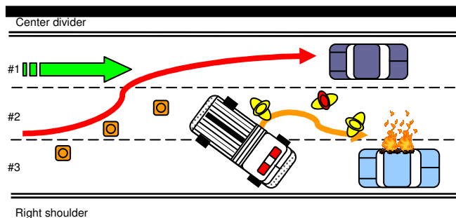
Figure #2 – Engine has “blocked right.” Note the “shadow” where crews can safely operate and deploy hose lines.
