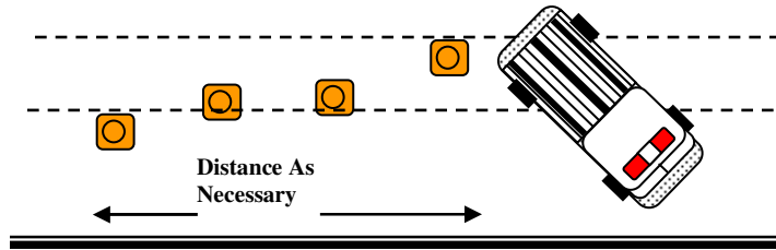
Figure #5 – The greater the traffic speed, the greater the upstream distance for cone placement.
